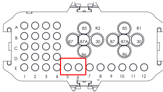
FIG 2-HVAC FUSE TERMINAL INSERTION VIEW
