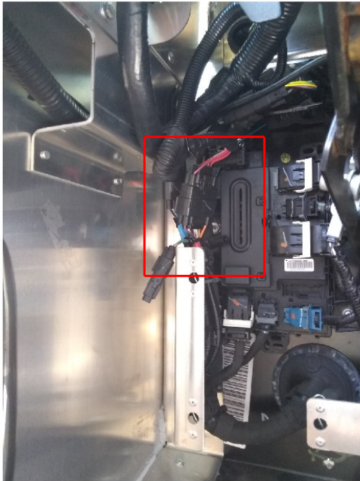
FIG 1 - HVAC POWER SOURCE FROM F59 CHASSIS
